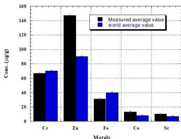
Fig. 2: Comparison of the average metal concentration in the studied soil samples with the worldwide average value. (Fe concentration values are divided by 1000).
