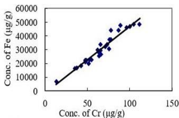
Fig. 3: Correlation between Cr-Fe
