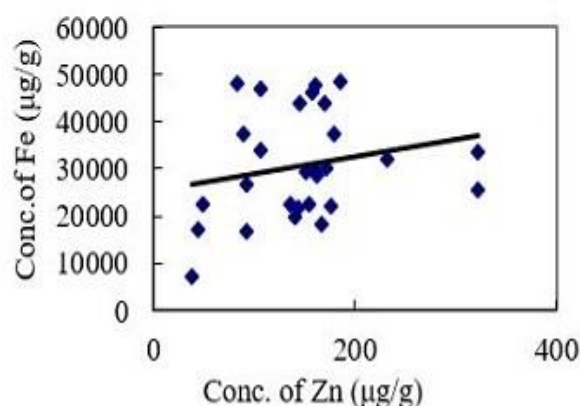
Fig. 4: Correlation between Zn-Fe
