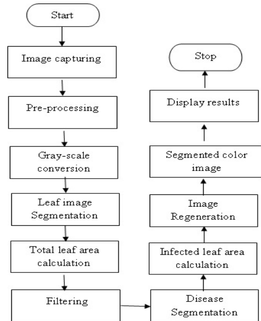
Figure 1. Flow chart of the SACD algorithm
