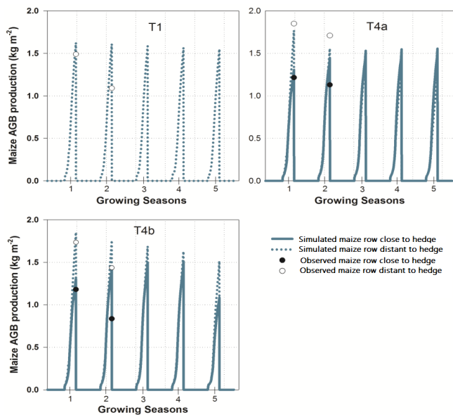
Figure 2. Simulated options for sustainable maize production in agroforestry systems with five growing seasons. Growing seasons 1 & 2 are also showing AGB observed values from 2010 and 2011 field experiments, respectively.
