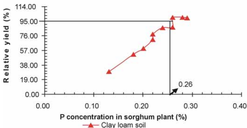
Fig 2. Internal P requirement of sorghum fodder
