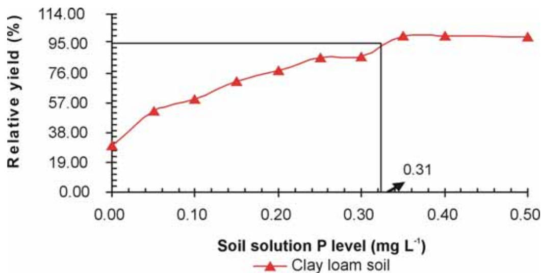
Fig. 1. External P requirement of sorghum fodder
