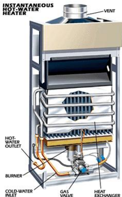
Figure 2: Instant Water Heater (Source: Klenck, T: 1997)
