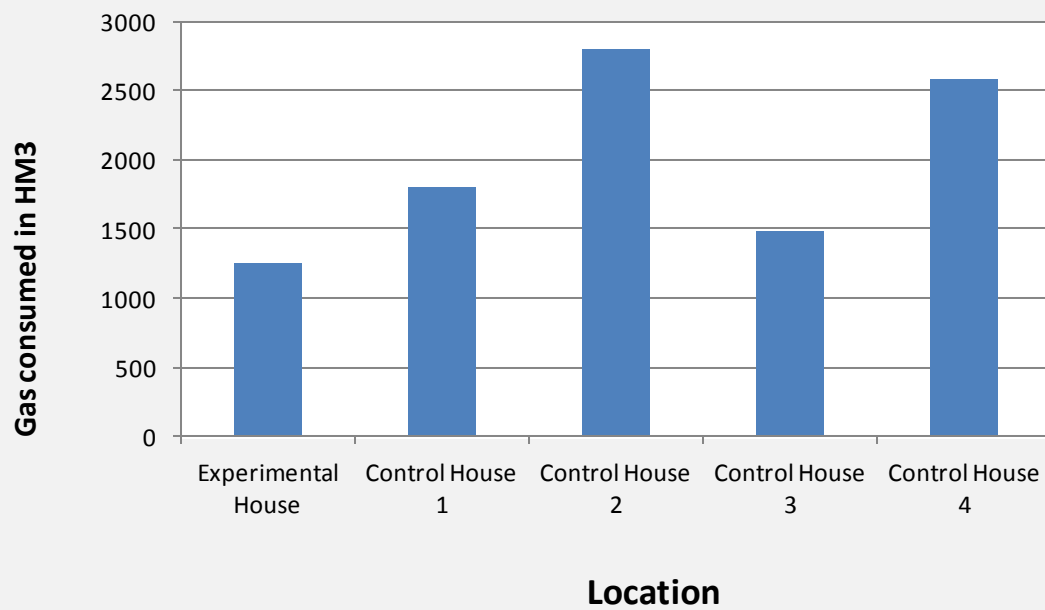
Figure 4: Average Monthly Gas Consumption With Geyser In Use
