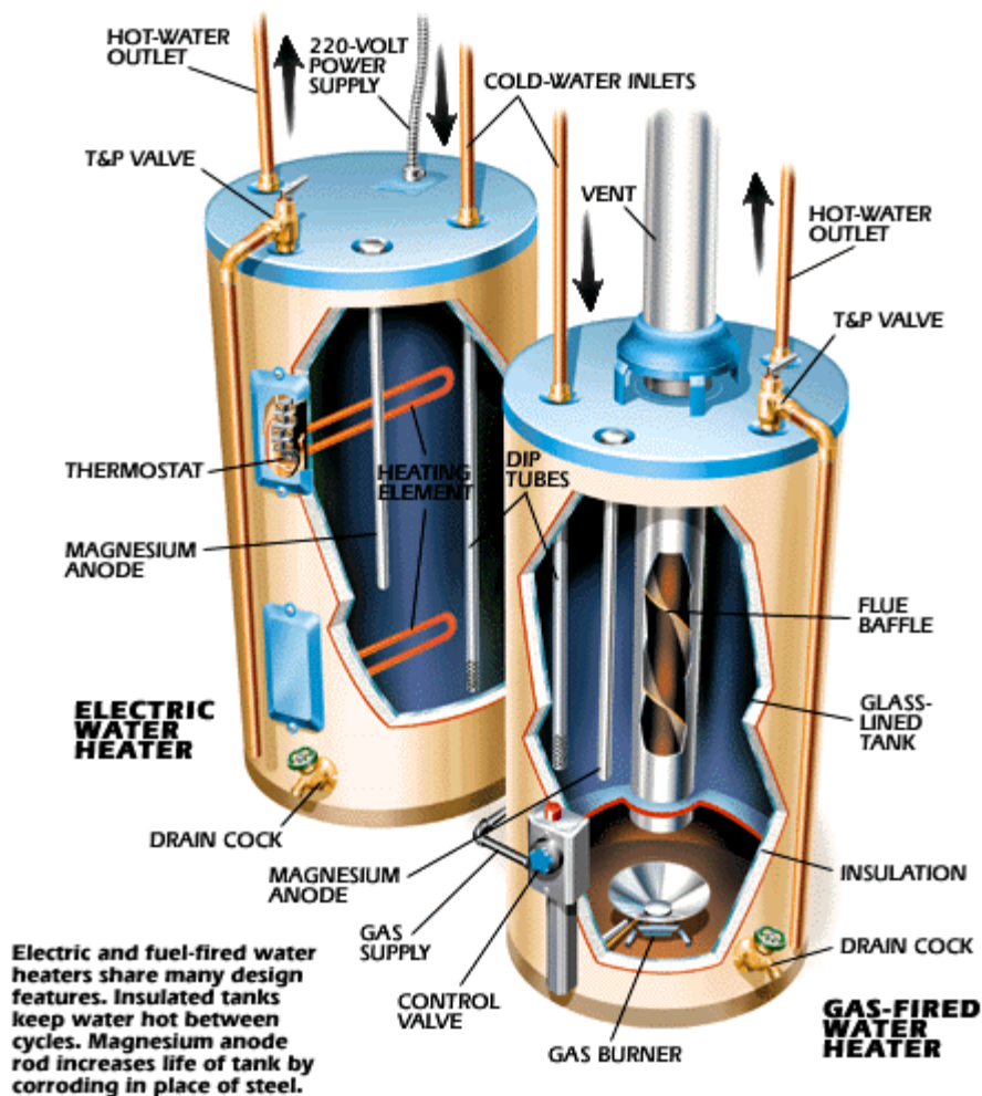
Figure 1: Conventional water heater (source: Klenck, T: 1997)
