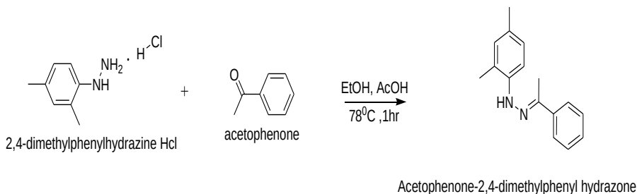
Scheme 3: Synthesis of acetophenone-2, 4-dimethylphenyl hydrazone (3)
