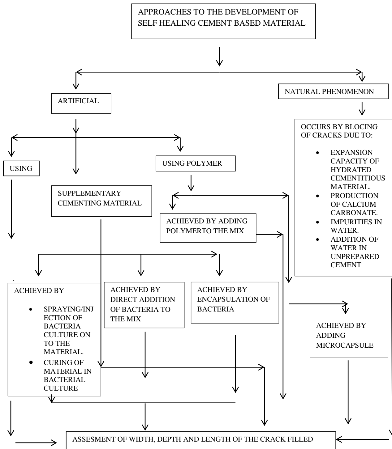
Fig. 1. Research based taxonomy of cement material (Muhammad et al. , 2016).
