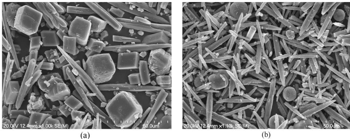
Fig. 2. (a) Scanning Electron Microscopy (SEM) image that shows the formation of calcite precipitate by Bacillus sphaericus . (b) SEM image that shows the formation of calcite precipitate by Bacillus subtilis . (Wiktor and Jonkers, 2011; Jonkers et al. , 2010).
