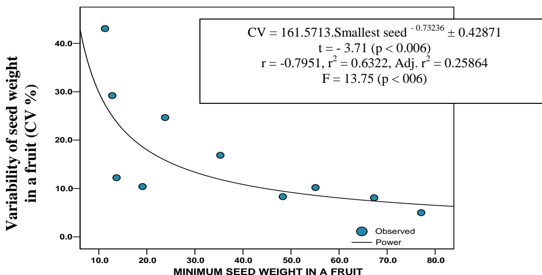
Fig. 4. Relationship of Seed weight variability in fruits of L. cylindrica with the lowest weight seed of the fruits.
