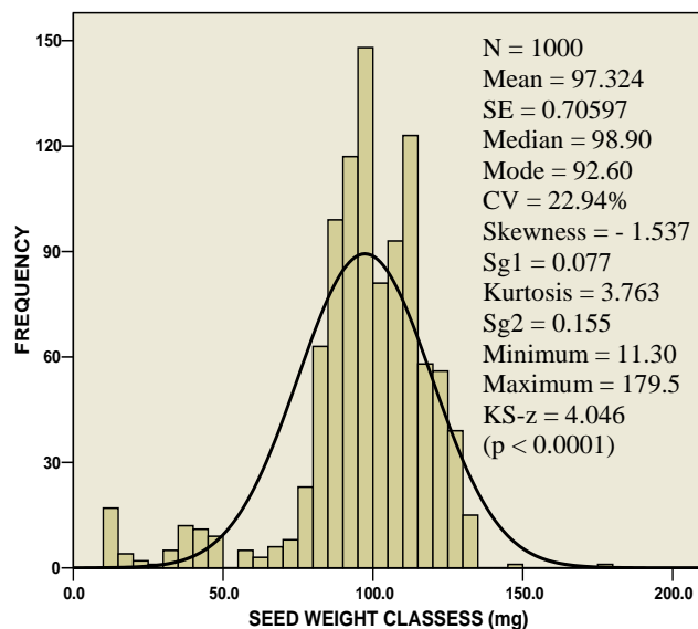
Fig. 5. Frequency distribution of seed weight (mg) of composite seed sample of Luffa cylindrica .
