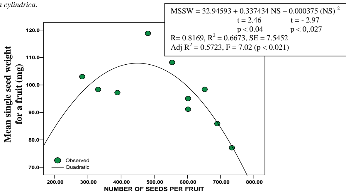
Fig. 3. Relationship of Mean single seed weight (MSSW) for a fruit of Luffa cylindrica with number of seeds per fruit. The relationship is quadratic.
