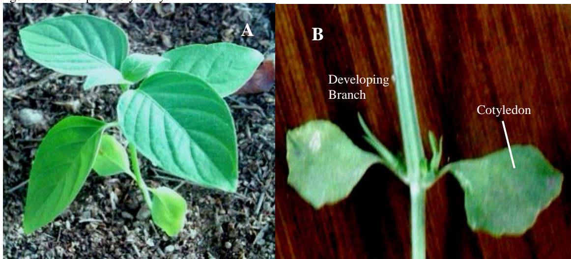
Fig. 1. A, Nearly one month old seedling of P. paniculata growing in a derelict site of Karachi University. Cotyledons are still intact. Photo Aug. 2015. The leaves are pinnately veined. The midribs as well as the secondaries run in depression. Fig. 1B exhibits the branch shoots arising from the axil of the cotyledons. Stem is angular with ridges and grooves.
