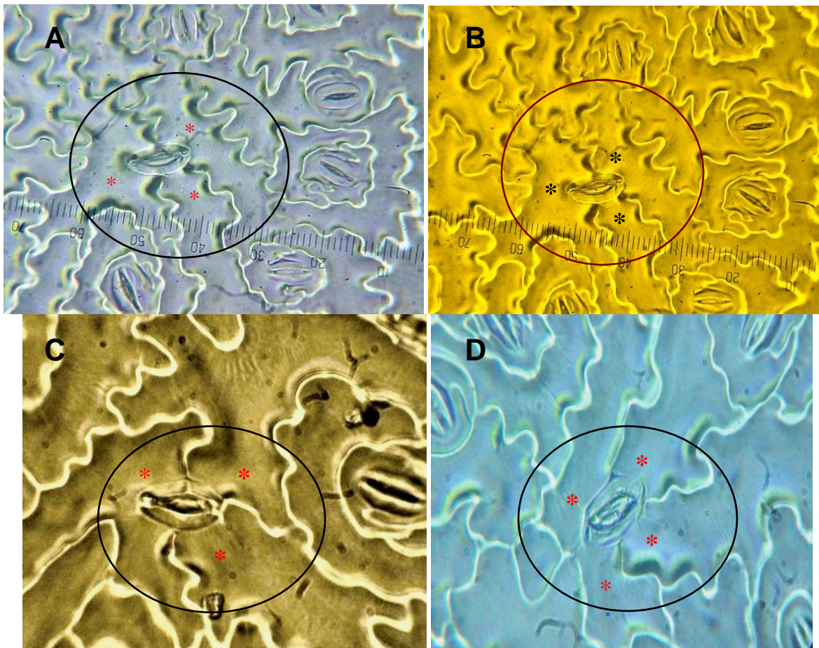
Fig. 15. Anisocytic (A, B and C) and staurocytic type of stoma (D) on the ventral surface of P. paniculata leaf. Some ten instances of occurrence of such stomatal types were recorded. Images: 45 x10 X.
