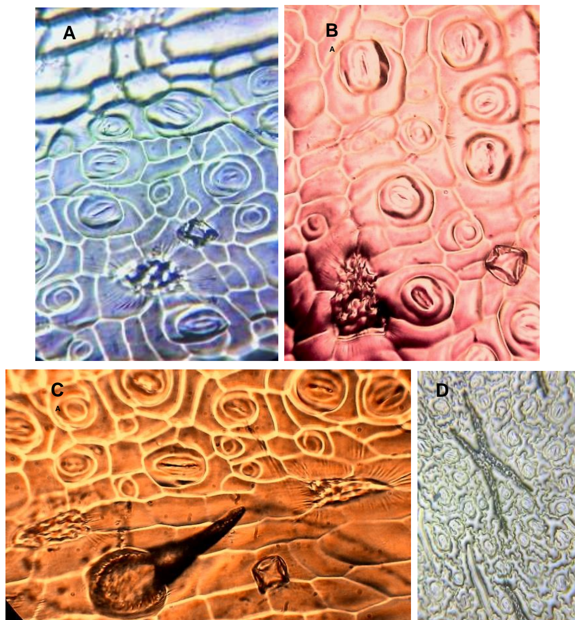
Fig. 10. Surface of epicotyl showing meristemoids, stomata, trichomes and crystals and differentiation of groove and ridge cells. Ridge bears more trichomes (A, B and C). The crystals are presumably of calcium oxalate. Two bent lithocysts are seen to join to form X-shaped structure (D). Images A-C: 45 x 10 X. Image D: 10x10 X.
