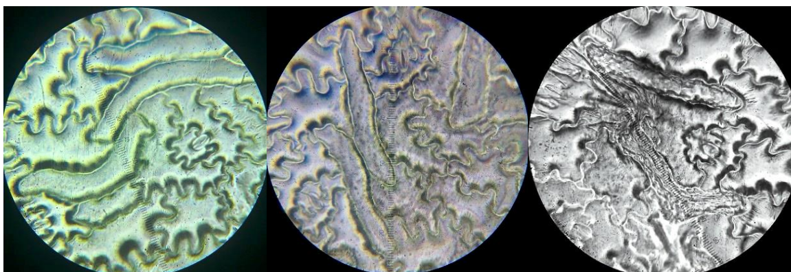
Fig. 6. P. paniculata cotyledon dorsal surface. Progressively developing lithocysts.
