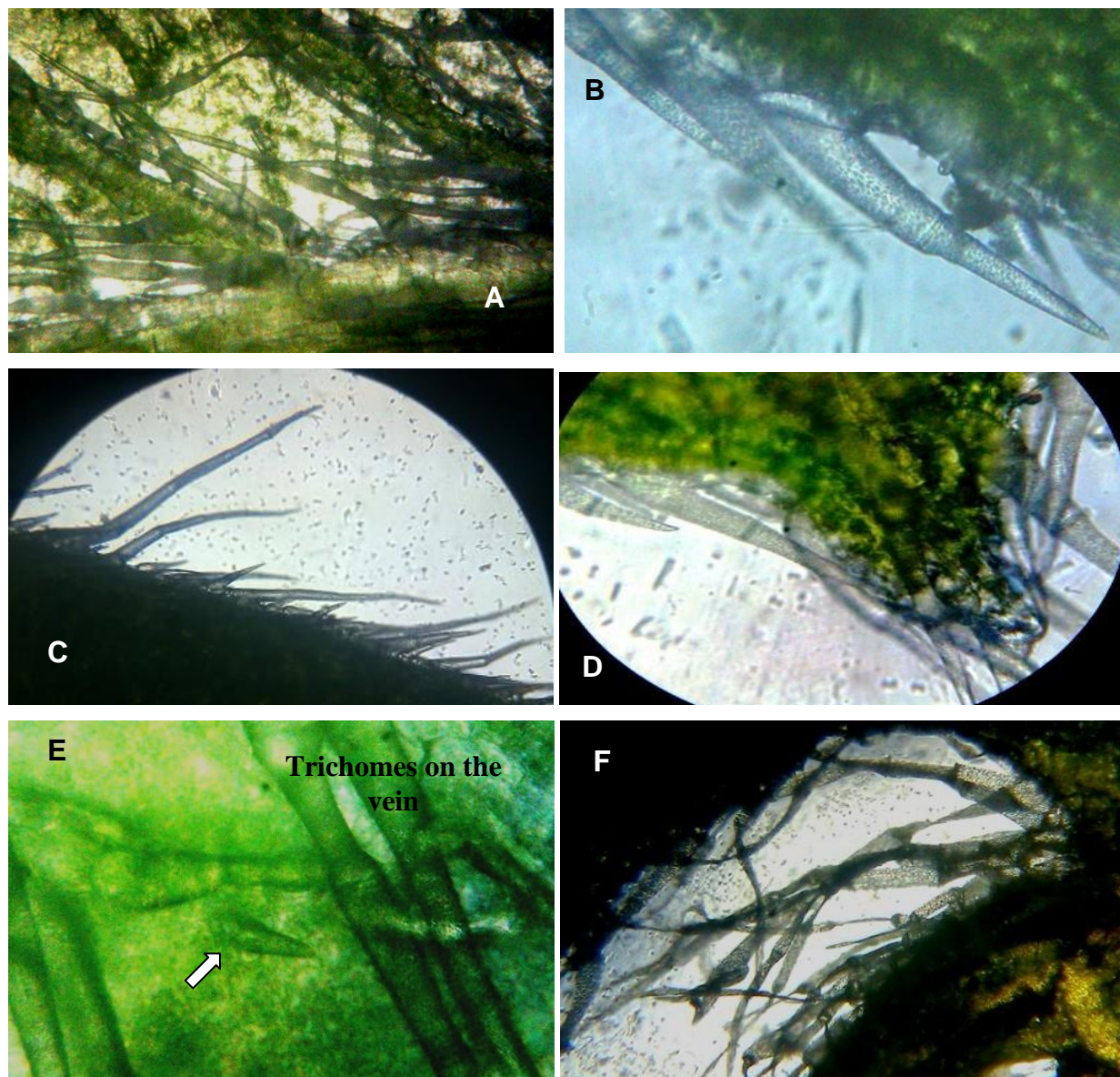
Fig. 2. Multicellular trichomes (2-6 or more celled) of P. paniculata leaf as seen under optical microscope. A, midrib and sub-vein region (ventral) B, Lower margin of the leaf; C, Upper margin; D, Apex; E, Laminar island (Arrow indicates the small conical stout trichome); F, Umbo region of the leaf (petiole visible).
