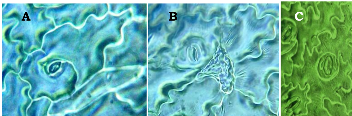
Fig. 17. An abnormal stoma (A) and a lithocyst (B) close to a diacytic stoma on the dorsal surface of leaf. (C) - a smaller foliar stoma surrounded by smooth walled subsidiaries and then a cycle of two normal sinuous subsidiaries. Photos: OM (45x10 X)
