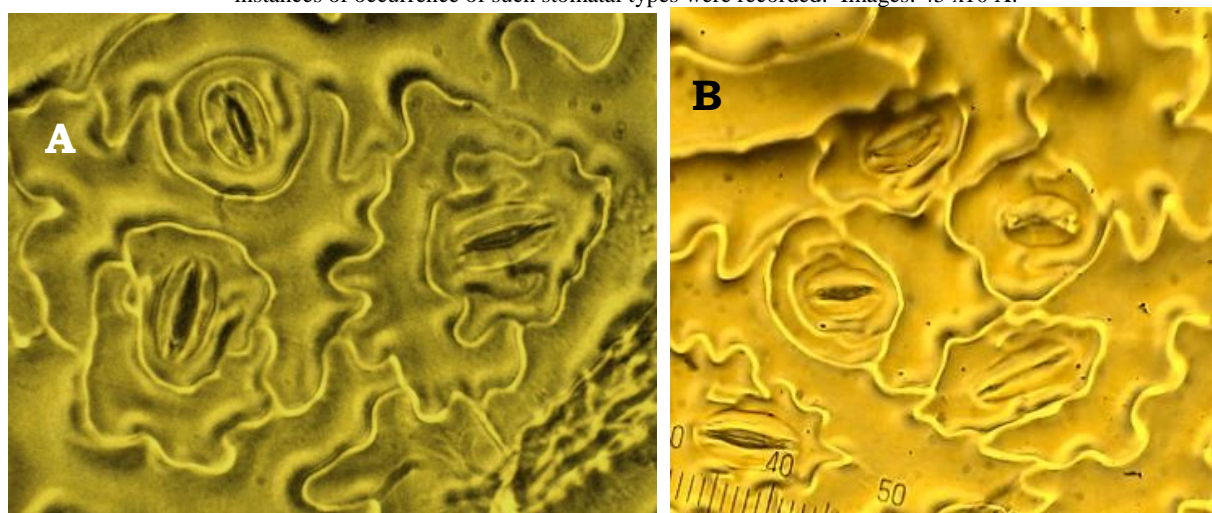
Fig. 16. A cluster of three and four stomata on dorsal surface of leaf. (Photos: 45x10 X).
