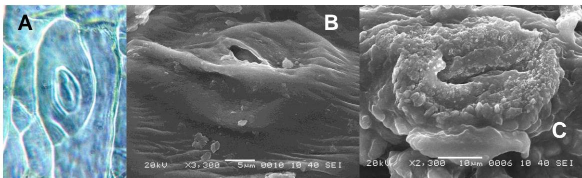
Fig. 11. Three hypocotylar stomata. A, OM image; B and C, SEM images. Thick epicuticular and other deposits apparent particularly in image C –stoma from basal region of hypocotyl. Diacytic nature apparent from image A.
