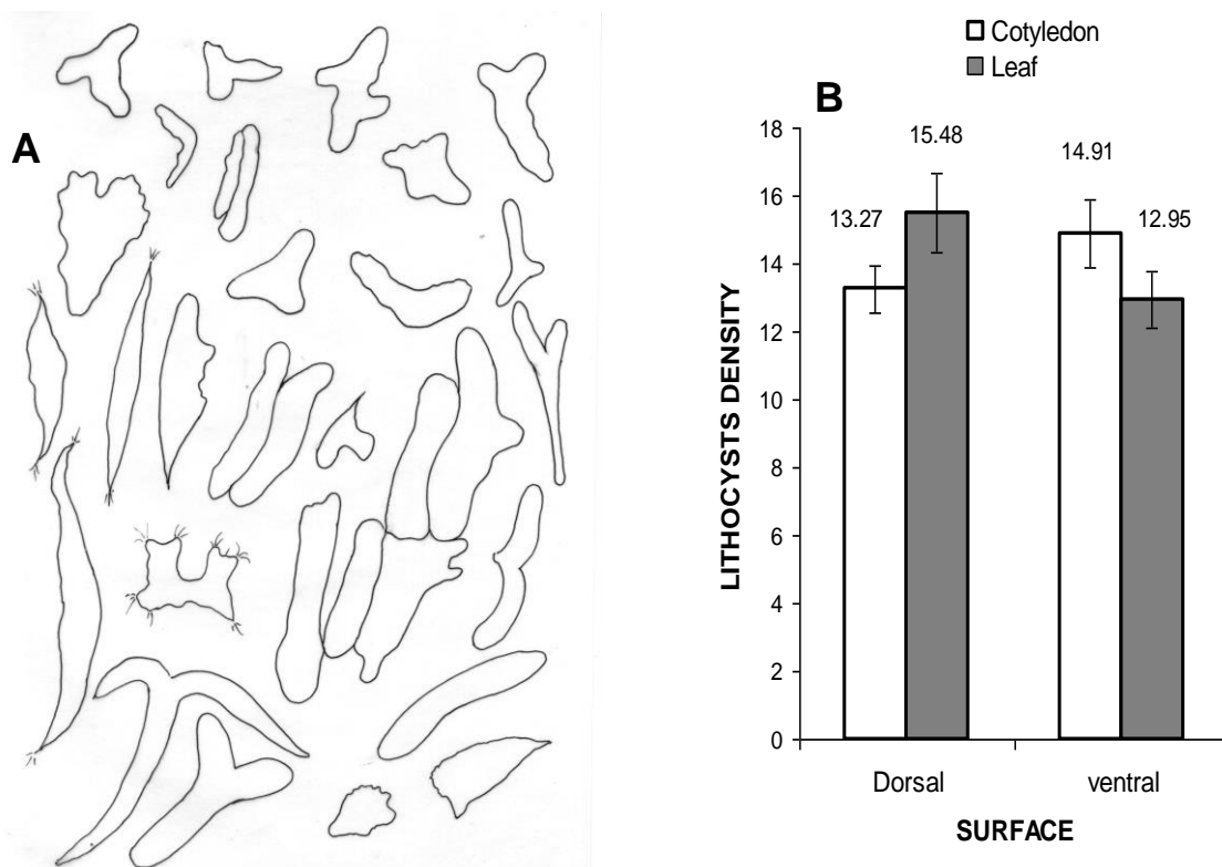
Fig.5. A) Free hand illustration of few of the variously shaped lithocysts of P. paniculata hypocotyl, cotyledons and leaf. Figures are not drawn to scale and the cystoliths are not shown. B) The density. \text{mm}^{-2} of lithocysts on the surfaces of seedling cotyledon and the leaf.
