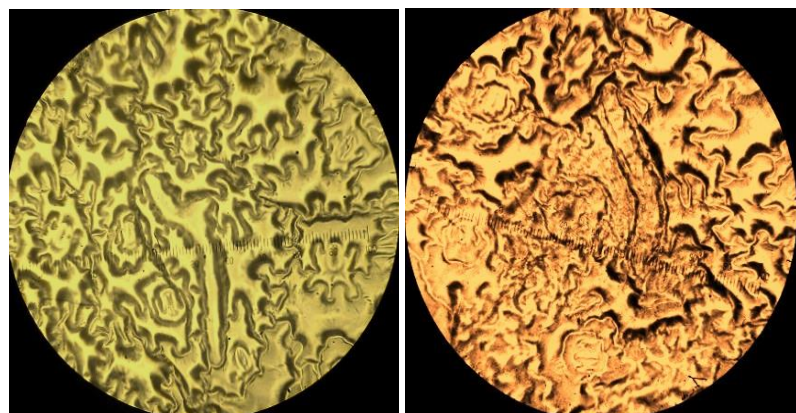
Fig. 8. Lithocysts from ventral surface of a young cotyledon. A, developing lithocyst and B, two fairly developed adjacent lithocyst.
