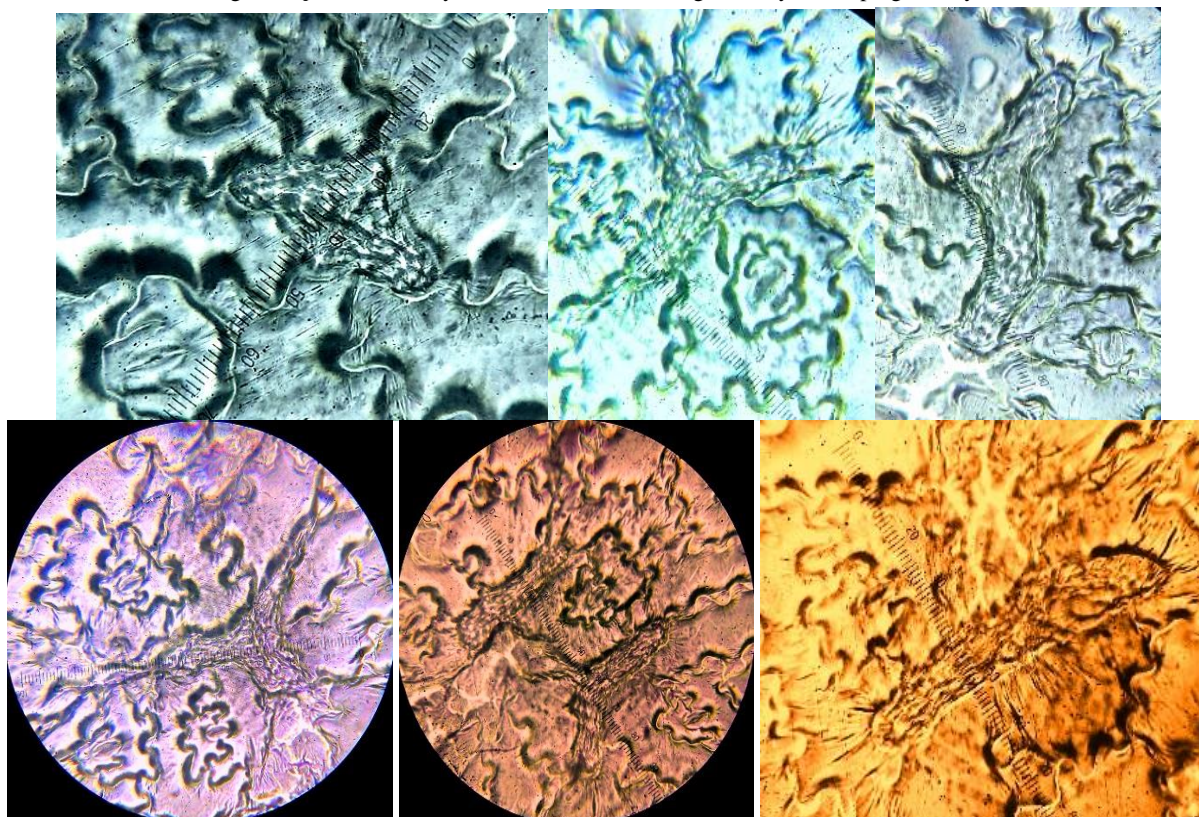
Fig. 7. Variously shaped lithocysts on dorsal surface of P. paniculata cotyledon.
