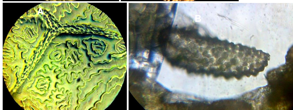
Fig. 9A. T-shaped lithocyst on ventral leaf surface. Fig. 9B. lithocyst separated from a mature leaf (45 x 15 X).
