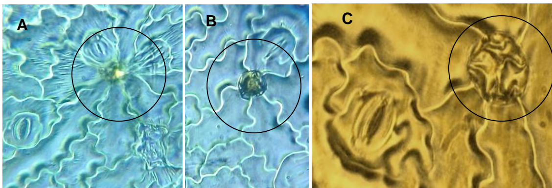
Fig.4. Sessile glandular trichome (SGT) on dorsal (A and B, 45x10X) and ventral surface (C) of leaf.(45x 15 X).
