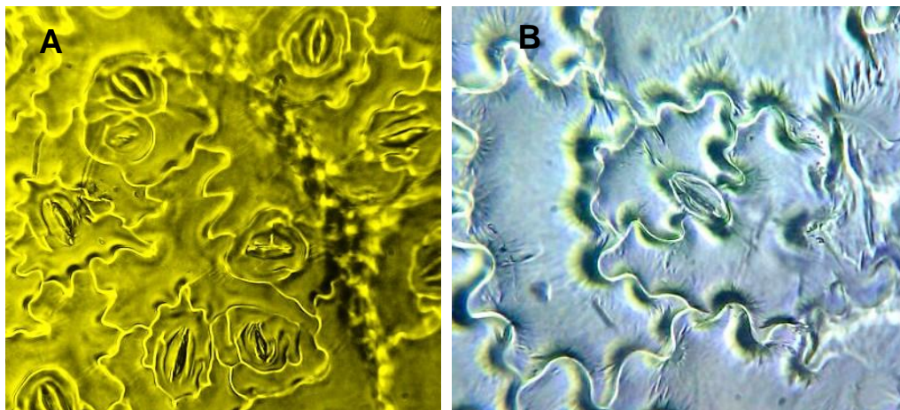
Fig. 13. The OM view of surface of fresh leaf. A, ventral surface view (45 x 10X). B, The enlarged view of the surface (45 x 15 X) to show single stomata and ground epidermal cells. The subsidiaries as well as the pavement epidermal cells are with wavy anticlinal walls.
