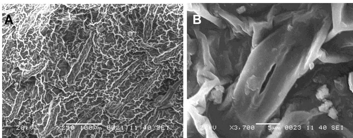
Fig. 12. General view of the dorsal surface showing a crop of lithocysts (A) and a stoma from the dorsal surface of leaf (B).
