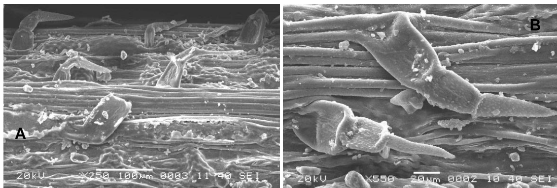
Fig. 3. SEM of epicotylar surface showing grooves, ridges, lithocyst and trichomes (A) and a Close up view of trichomes on epicotyl (B) showing basal connection.
