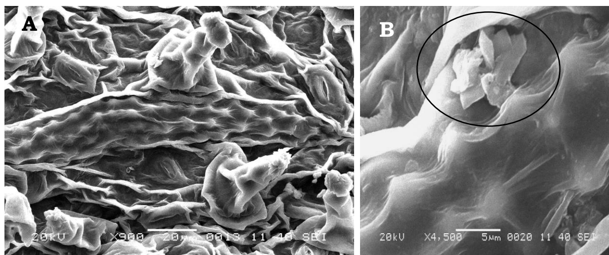
Fig. 18. (A) - Ventral surface of leaf showing trichomes, lithocyst containing cystoliths and stomata. Included inside lithocyst are several cystoliths formed due to the deposition of crystals of calcium salts being wrapped in cellulose. Note the erect trichomes with druses on the top. (B) SEM image of a crystals aggregate (aragonite type) nearby a lithocyst on the ventral surface of leaf. The wrapping of cystoliths inside cellulosic wall is apparent.
