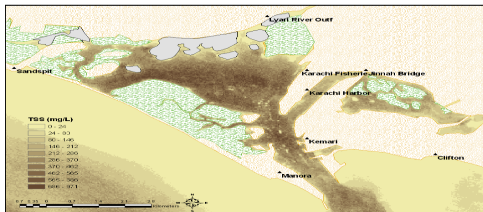
Fig 6. Model derived density-sliced map of TSS.
