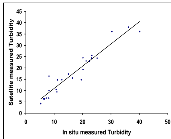
Fig. 3. Linear regression of satellite estimated Turbidity vs. in situ measured Turbidity of water in three TM bands.
