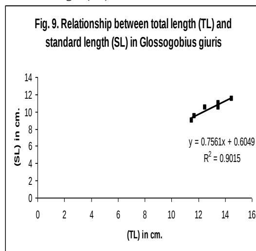
Fig.9. Relationship between total length (TL) and standard length (SL) in Glossogobius giuris .
