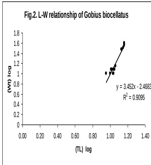
Fig.2. L-W relationship of Gobius biocellatus .
