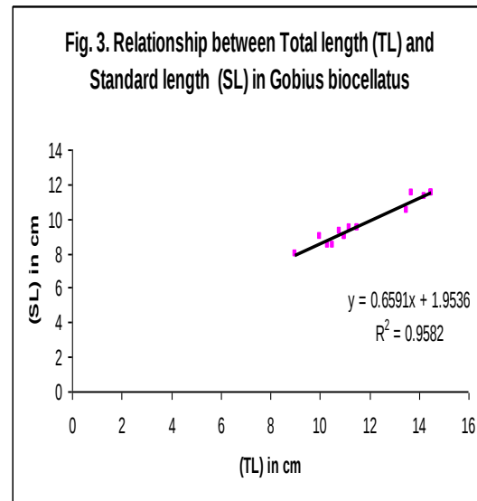
Fig.3. Relationship between total length (TL) and standard length (SL) in Gobius biocellatus .
