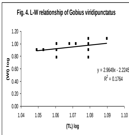
Fig.4. L-W relationship of Gobius viridipunctatus .
