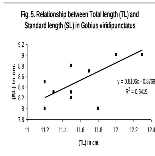
Fig.5. Relationship between total length (TL) and standard length (SL) in Gobius viridipunctatus .
