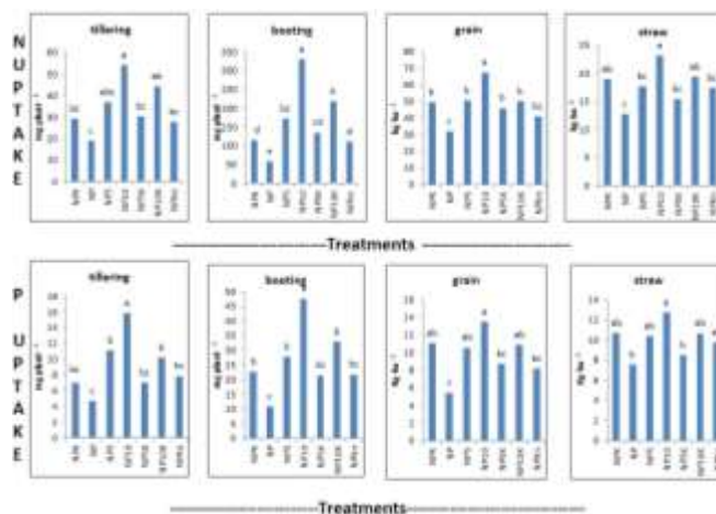
Figure 1. Effect of different combinations of nano coated and uncoated fertilizers on N and P uptake in shoot (at tillering and booting stage) and in grain and straw (at harvesting), significant at p \leq 0.05 .
