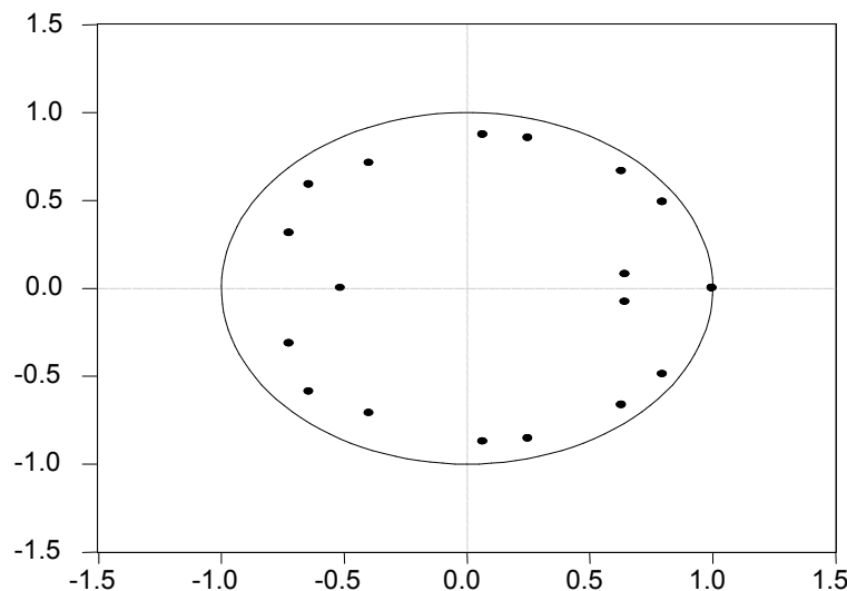
Figure-1: VECM Characteristic Roots
