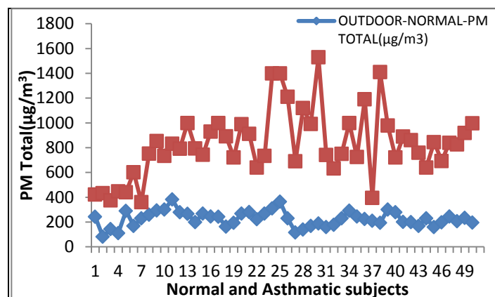
Fig. 6: PM Total concentration (outdoor) of normal and asthmatic subjects.
